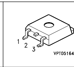
PG-TO263-3-2
